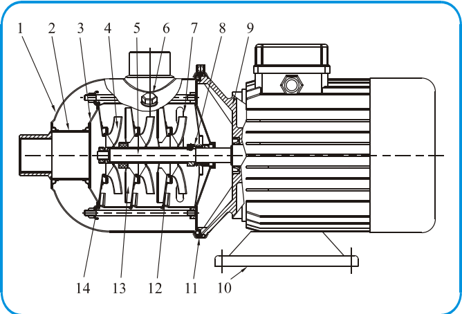
截面图 CHL, CHLK8,12,16,20
